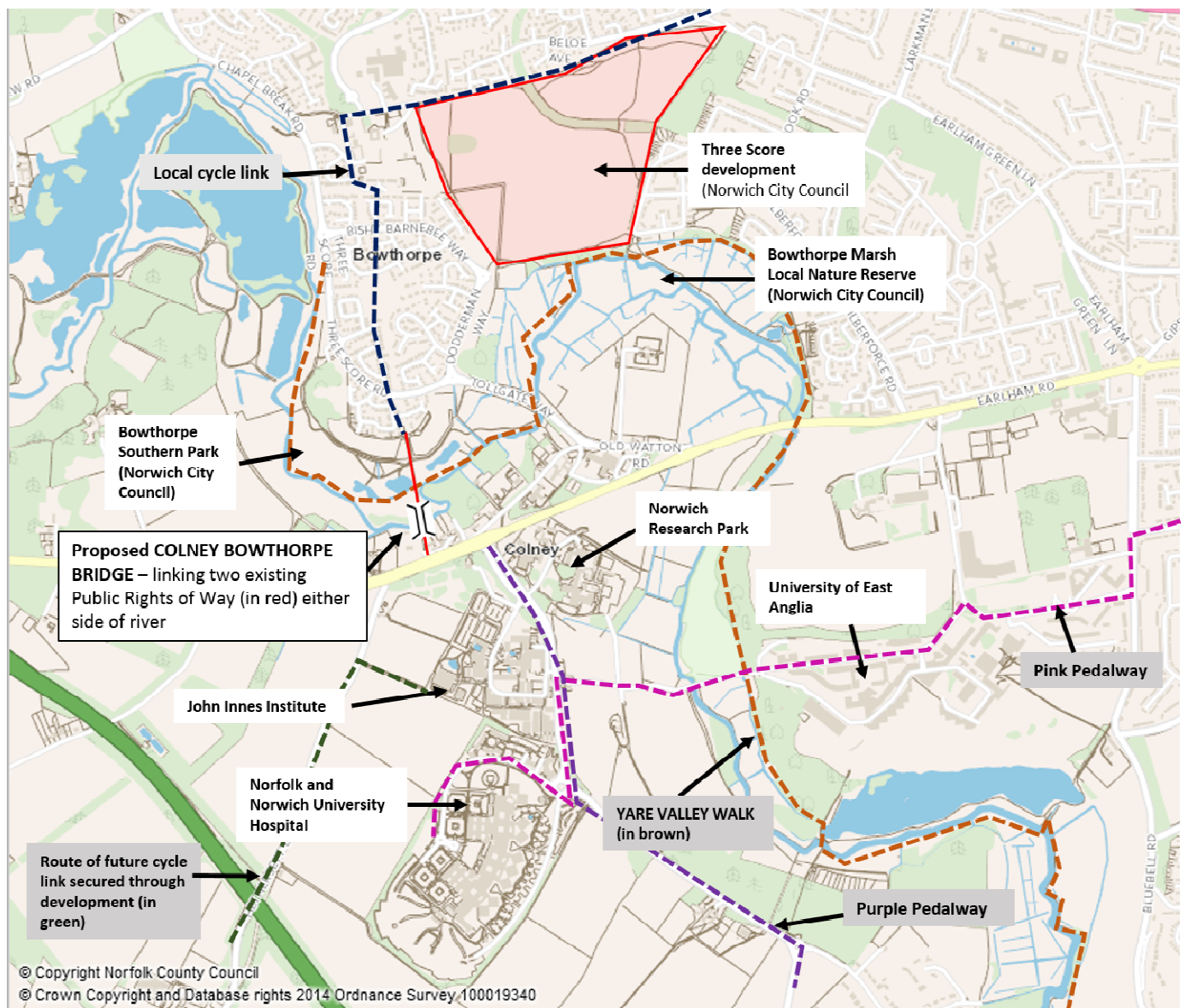
Plan 2 (below) showing the location of the bridge in context of local infrastructure
